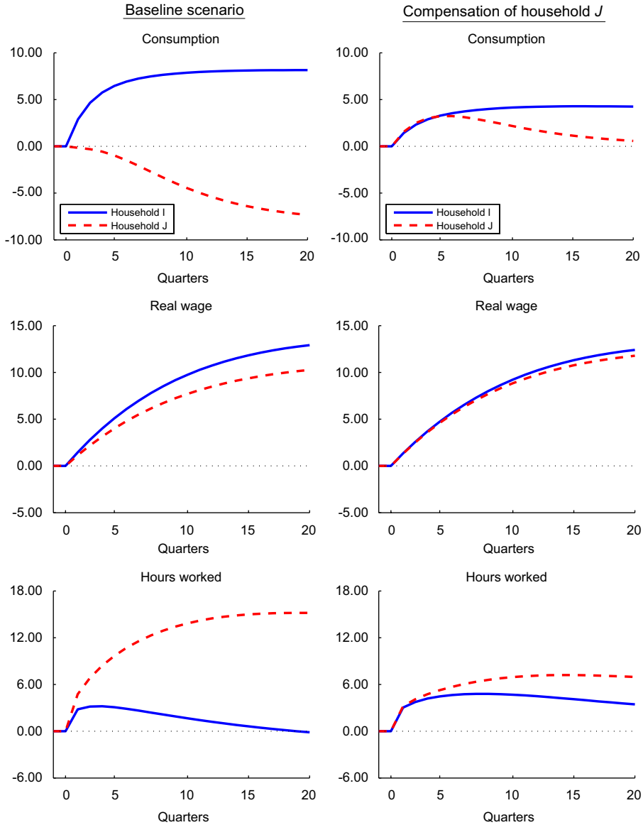
Fig. 6. Distributional effects of a gradual reduction in non-wage labour cost. Notes: For the baseline version of the NAWM, this figure depicts the distributional effects on selected household-specific variables of a gradually phased-in permanent reduction in firms' social security contributions from 21.9% to 7.1% under alternative assumptions regarding burden sharing amongst households. All dynamic effects are reported as percentage deviations from steady state.
