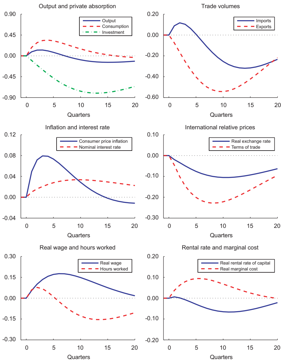
Fig. 3. Dynamic responses to a transfer shock. Notes: For the baseline version of the NAWM, this figure depicts the dynamic responses of selected domestic variables to a persistent transfer shock ( \rho_{tr} = 0.90 ) equal to an 1% increase in steady-state output. All dynamic responses are reported as percentage deviations from steady state, except for the dynamic responses of inflation and the interest rate which are reported as percentage-point deviations.
