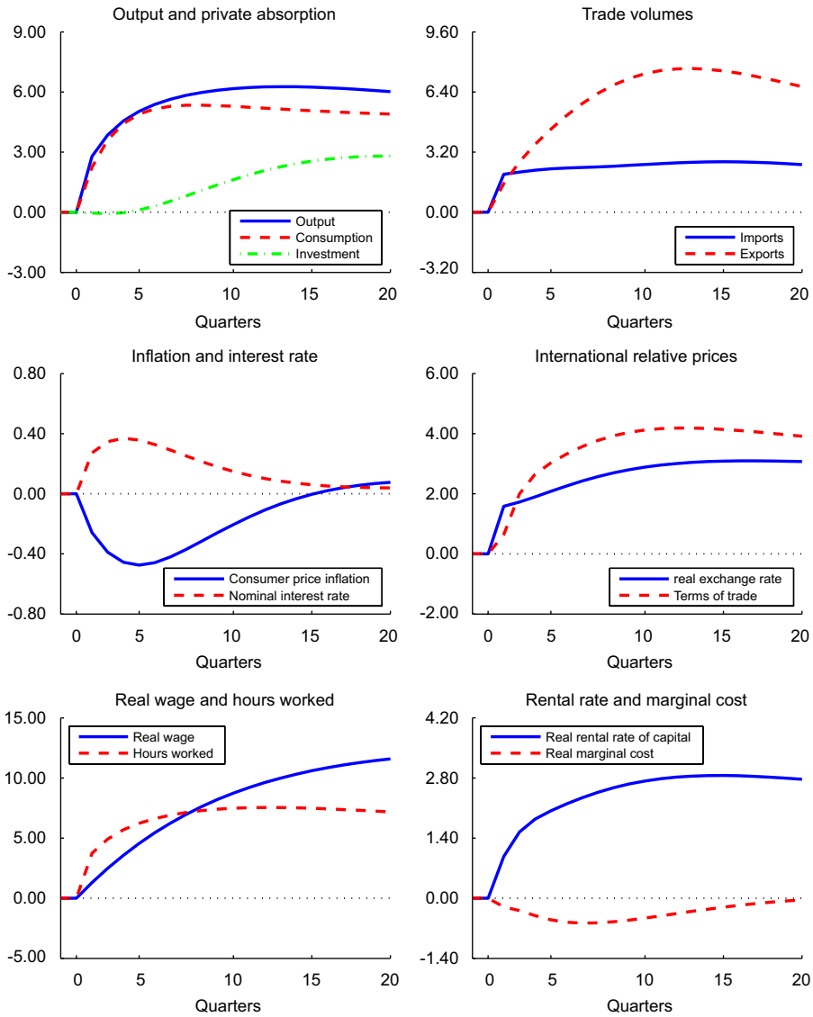
Fig. 5. Transitional dynamics after a gradual reduction in non-wage labour cost. Notes: For the baseline version of the NAWM, this figure depicts the transitional dynamics of selected domestic variables after a gradually phased-in permanent reduction in firms’ social security contributions from 21.9% to 7.1%. All dynamic effects are reported as percentage deviations from the initial steady state, except for the dynamic responses of inflation and the interest rate which are reported as percentage-point deviations.
