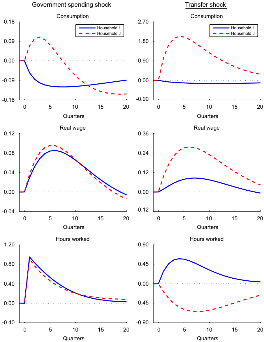
Fig. 4. Household-specific responses to fiscal policy shocks. Notes: For the baseline version of the NAWM, this figure depicts the dynamic responses of selected domestic variables to a government spending shock and a lump-sum transfer shock, equal to a 1% increase in steady-state output. All dynamic responses are reported as percentage deviations from steady state.
