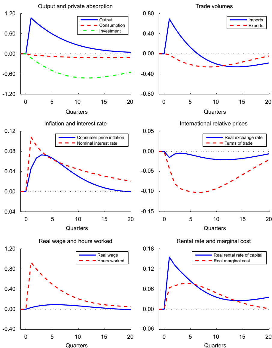
Fig. 2. Dynamic responses to a government spending shock. Notes: For the baseline version of the NAWM, this figure depicts the dynamic responses of selected domestic variables to a persistent government spending shock ( \rho_g = 0.90 ) equal to a 1% increase in steady-state output. All dynamic responses are reported as percentage deviations from steady state, except for the dynamic responses of inflation and the interest rate which are reported as percentage-point deviations.
